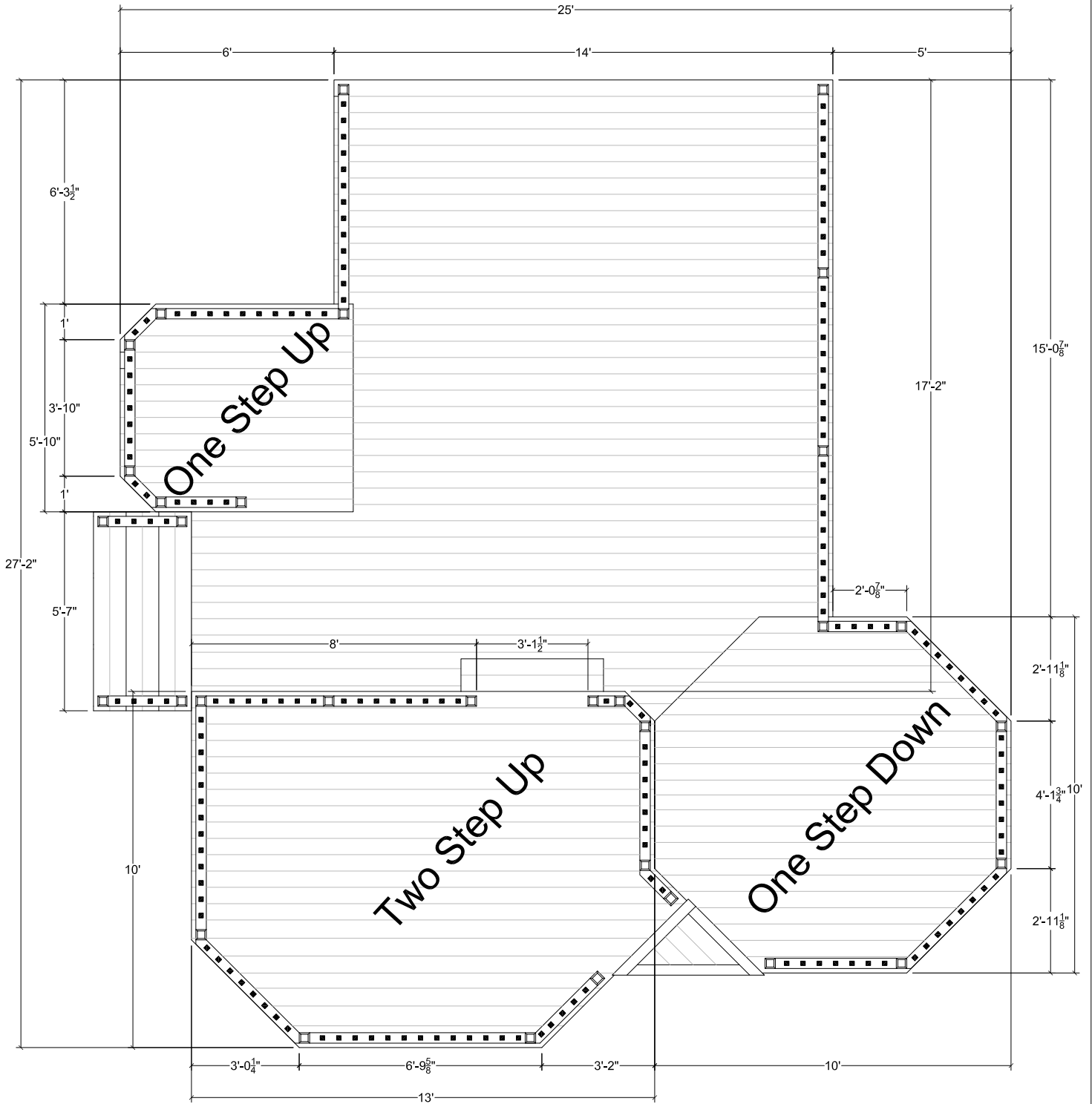
1 Deck Plan Scale: 1/4" = 1'-0"
